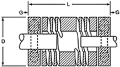
Flexible Helical Couplings
