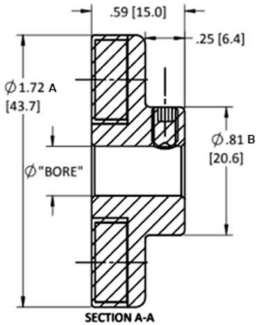
Magnetic Coupling
