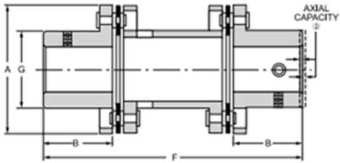
Flexible Disc Couplings
